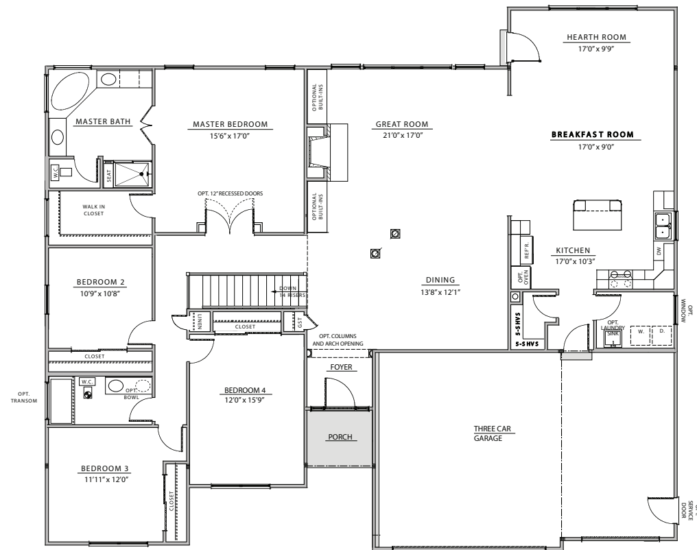
MAIN LEVEL WITH OPTIONAL 4TH BEDROOM
